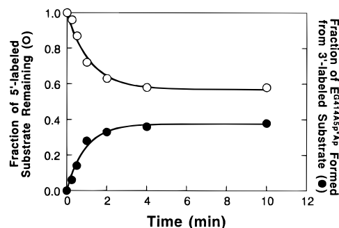
FIGURE 3: L-21G414 ribozyme reaction reaches a plateau. Reactions of 100 \text{ nM} \text{E}^{\text{G414}} with 0.1 \text{ nM} 5'-labeled -1\text{d},\text{rS} ( \text{p}^*\text{CCCUCdUA}_5 ) (○) or 3'-labeled -1\text{d},\text{rS} ( \text{CCCUCdUA}_5\text{p}^*\text{Ap} ) (●) with 10 \text{ mM} \text{MgCl}_2 and 50 \text{ mM} sodium MES (pH 6.8) at 50^\circ\text{C} . Lines represent nonlinear least-squares fits to the data with k_{\text{obs}} = 0.90 \text{ min}^{-1} and an endpoint of 0.6 for disappearance of the 5'-labeled substrate (○) and k_{\text{obs}} = 0.95 \text{ min}^{-1} and an endpoint of 0.4 for formation of the 3'-labeled product, \text{E}^{\text{G414A}_5\text{p}^*\text{Ap}} , from the 3'-labeled substrate (●).
