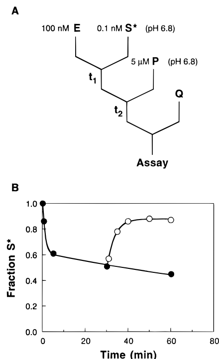
FIGURE 4: Regeneration of S* provides evidence for the establishment of the internal equilibrium ( K_{\text{int}} ). (A) Outline of the pulse chase protocol. E G414 (100 nM) was mixed with ~0.1 nM 5'-labeled -1d,rS* for t_1 = 30 min (10 mM MgCl 2 and 50 mM sodium MES, pH 6.8, at 50 °C). The reaction mixture was then diluted 10-fold by a chase solution containing 5 μM unlabeled rP to initiate the t_2 phase of the reaction. (B) The disappearance of S* during t_1 (●), and its regeneration during t_2 (○). The lines represent nonlinear least-squares fits to the data. The regeneration of S* during t_2 (○) follows a single first-order rate constant with k_{\text{obs}} = 0.28 \text{ min}^{-1} and an endpoint of 0.88 S*. The disappearance of S* during t_1 (●, additional time points not shown) is fit to two successive exponential functions according to the equation S_t = S_1 e^{-k_1 t} + S_2 e^{-k_2 t} , with k_1 = 0.88 \text{ min}^{-1} , k_2 = 0.005 \text{ min}^{-1} , S_1 = 0.38 , and S_2 = 0.62 . The initial fast phase represents establishment of the internal equilibrium and the second phase the slow dissociation of P (see text). (These values are in reasonable agreement with those obtained via independent approaches.)
