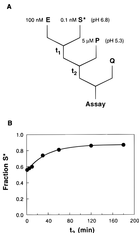
FIGURE 5: Determination of the rate constant for the reverse reaction ( k_r ). (A) E^{G414} was incubated with -1d,rS^* for t_1 = 10 min (10 mM MgCl_2 and 50 mM sodium MES, pH 6.8, at 50 °C). The reaction mixture was then diluted 10-fold with a low-pH chase solution containing 5 \mu M unlabeled P, 10 mM MgCl_2 , and 50 mM sodium MES (pH 5.3). (B) Time course for regeneration of S^* following the chase. The curve is a nonlinear least-squares fit to the data and gives k_{obs} = 0.021 \text{ min}^{-1} .
